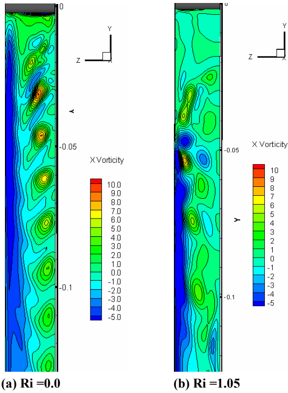
Figure 20. Instantaneous x-vorticity component at yz plane
