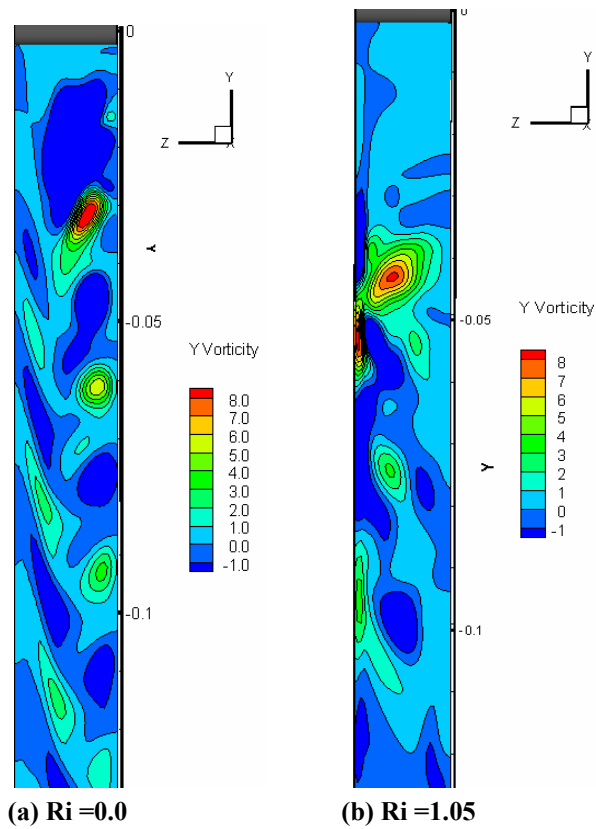
Figure 21. Instantaneous y-vorticity component at yz plane
