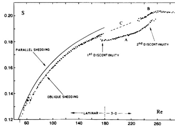
Figure 15. Strouhal-Reynolds number relationship over laminar and three-dimensional transition regimes Williamson [1]
