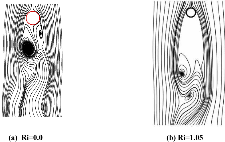
Figure 5. Computational Instantaneous streamlines
