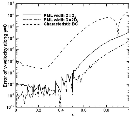
Figure 5: The error of v-velocity at time t = 2.0
