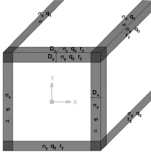
Figure 2: The schematics of the physical and PML domains (shadow). The sub-domains where the absorption coefficients are non-zero are indicated by arrows.
