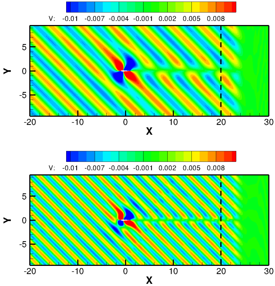
Figure 9: Instantaneous velocity contour, Y-component at wave number k = 1.0 (upper) and k = 2.0 (below)
