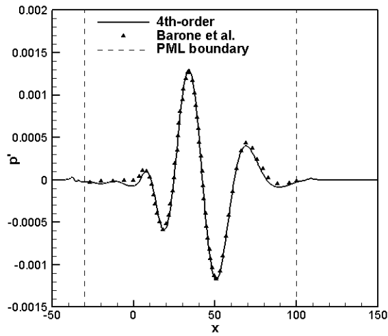
Figure 14 Pressure disturbances along the along y = -3 at t = 200
