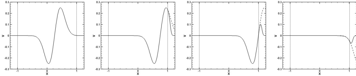
Figure 4: v-velocity profile along y=0 at time (a) t=0.5 , (b) t=1.5 , (c) t=2.0 and (d) t=3.0 (from left to right). Solid line: numerical solution; dashed line: exact solution
