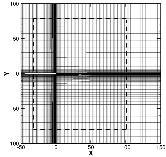
Figure 11 Computational mesh of Benchmark Problem 2
