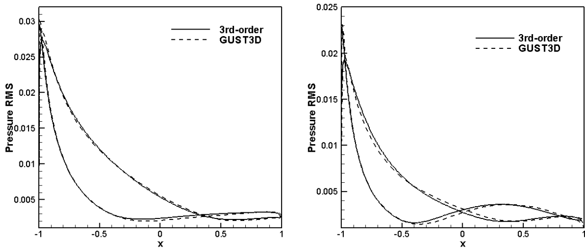
Figure 8: RMS pressure on the airfoil surface at wave number k = 1.0 (left) and k = 2.0 (right)
