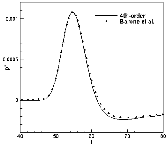
Figure 15 Acoustic pulse signals at (x, y) = (-30, 1)
