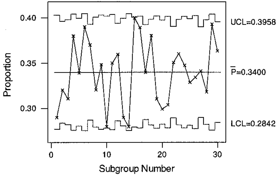
Accounts Payable P Chart for Proportion Defective
