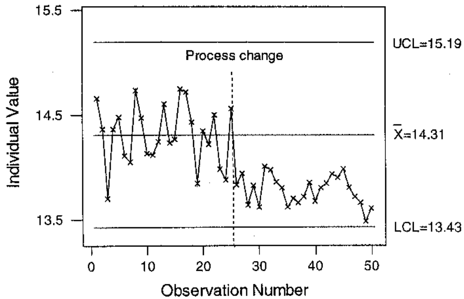
White Millbase Batch Process Individuals Chart (combined data)
