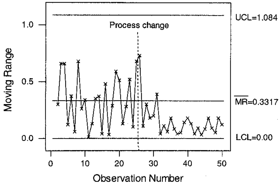
White Millbase Batch Process Moving Range Chart (combined data)
