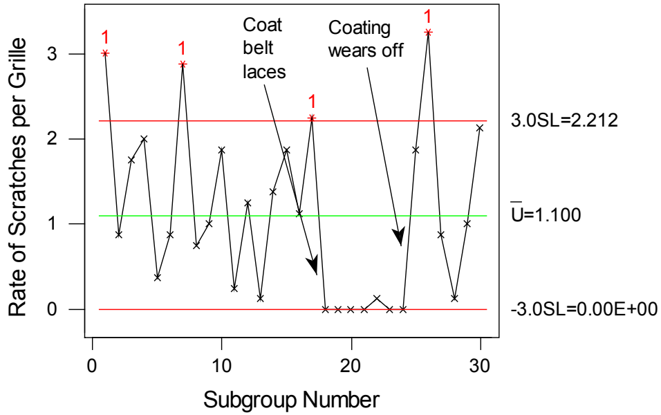
U chart (n=8)
