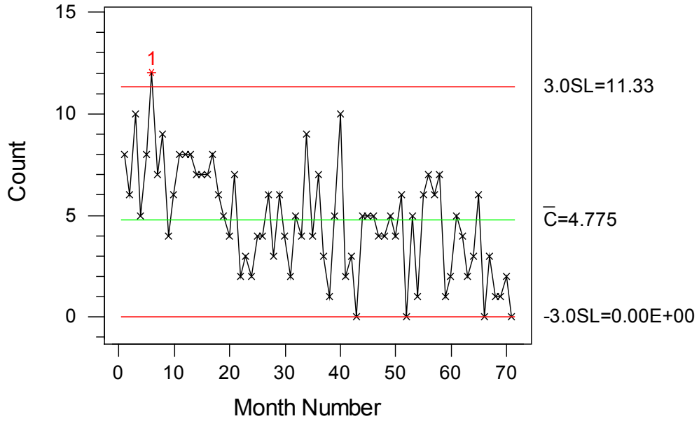
Accidents/Injuries per month c chart
