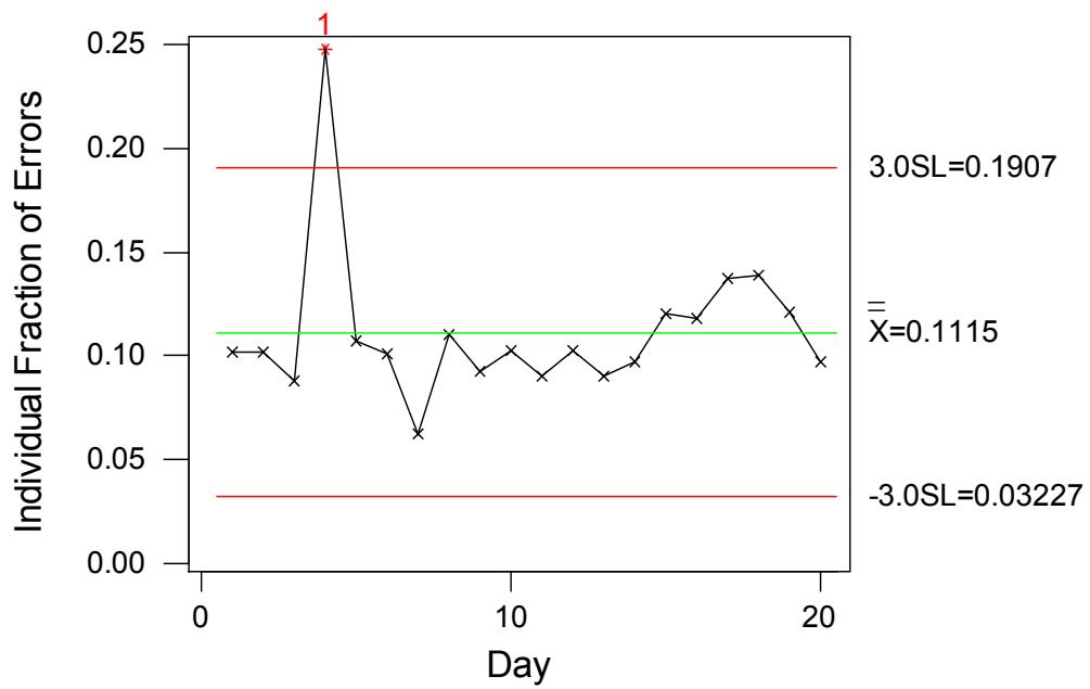
Internet Access Errors Individuals chart
