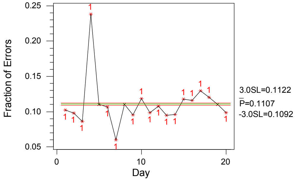
Internet Access Errors p chart
