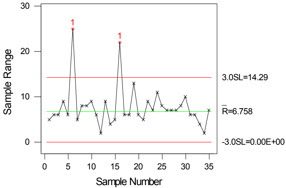
Cylinder Bore (subgroups 6 & 16 omitted) R chart
