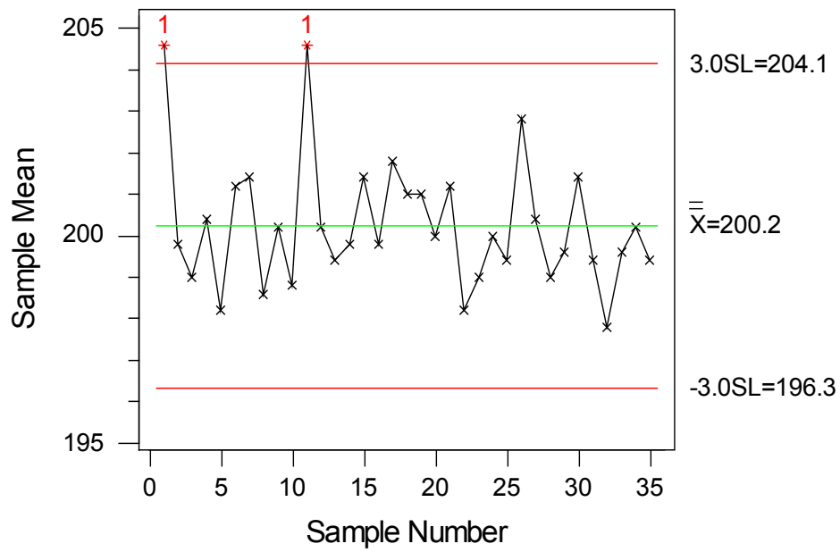
Cylinder Bore (subgroups 6 & 16 omitted) X-bar chart
