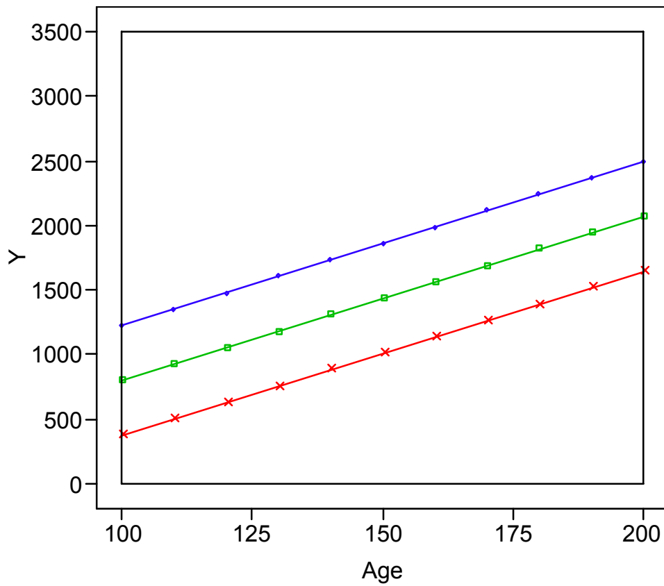
Plot of the no-interaction relationship between Age and Price (Y) for 5, 10 and 15 Bidders
