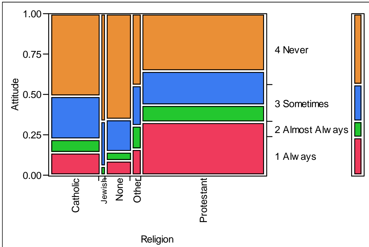
Contingency Table
