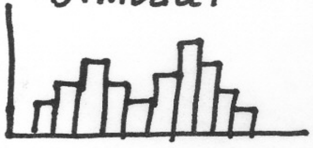
Bimodal
