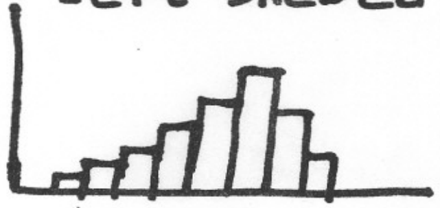
Left Skewed
