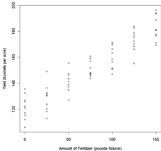
Yield of 10 Plots for each of 7 Fertilizer Amounts
