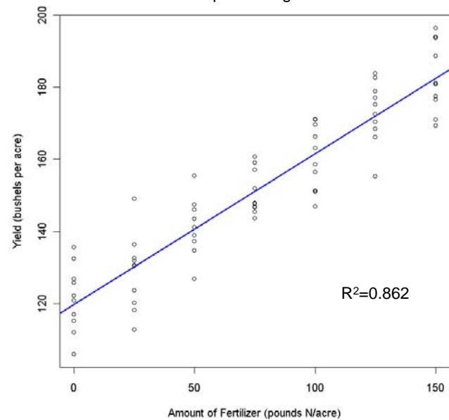
Scatter Plot of Yield vs. Amount of Fertilizer with Least-Squares Regression Line
