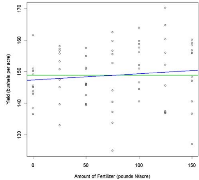
Least-Square Regression Line and Mean Yield
