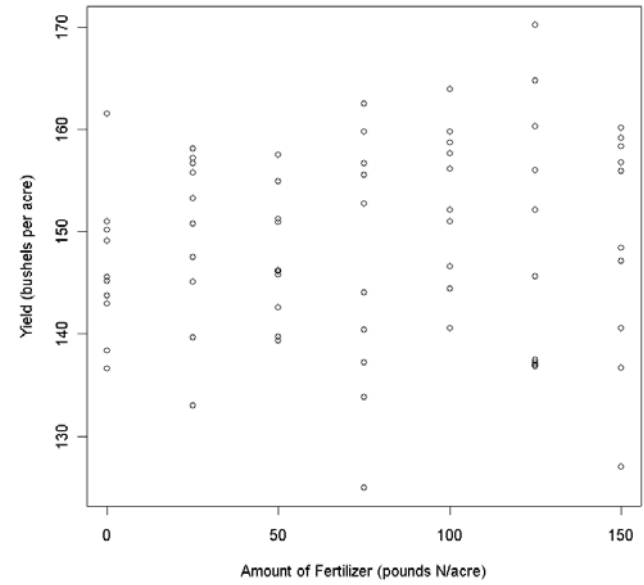
Yield of 10 Plots for each of 7 Fertilizer Amounts (2 nd Example)
