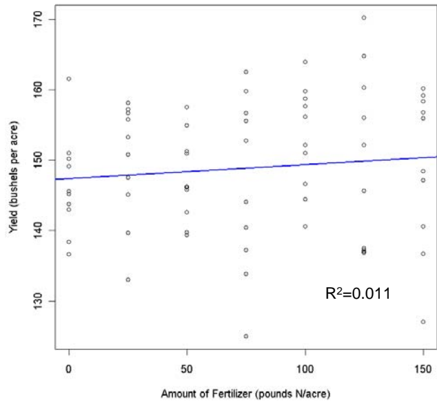
Scatter Plot of Yield vs. Amount of Fertilizer with Least-Squares Regression Line
