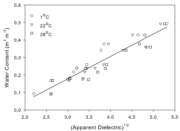
Figure 2. Volumetric soil moisture vs. Theta Probe response for laboratory calibration. The observed calibration equation is \theta = 0.118\sqrt{\epsilon} - 0.176 ( R^2 = 0.85 ).
