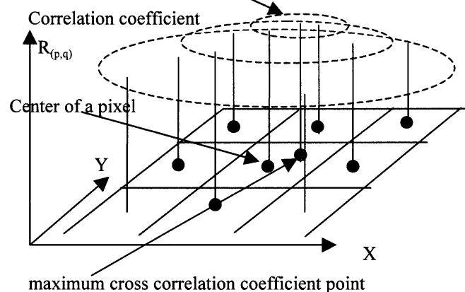
Fig. 7. The "sub-pixel interpolation" process.
