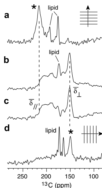
Fig. 3. ^{13}\text{C} O spectra of Val _{16} -labeled PG-1 in DLPC membrane. (a) 0^\circ -aligned spectrum from Ref. [7]. (b) Powder spectrum obtained with CP. (c) Difference spectrum after subtracting the lipid background signal, showing only the peptide signal. (d) Spectrum of a 90^\circ -aligned sample from Ref. [7]. The peptide signals in (a) and (d) are indicated by an asterisk.
