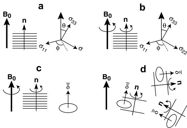
Fig. 1. Schematics showing the equivalence between the 0^\circ -aligned spectra and unoriented spectra. (a) Rigid 0^\circ -aligned sample. (b and c) Mobile aligned sample. In (c), the motionally averaged tensor has the unique axis along the bilayer normal. (d) Mobile unoriented sample.
