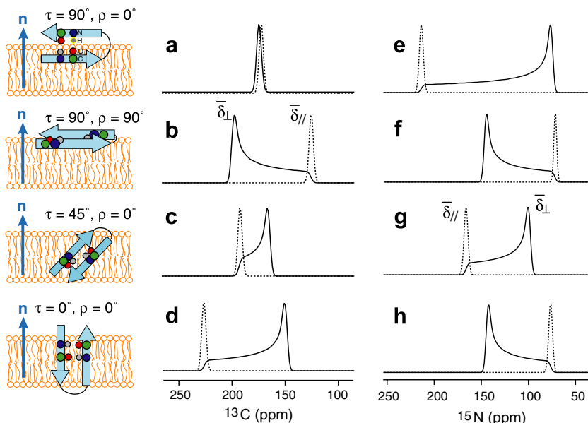
Fig. 2. Calculated ^{13}\text{C} O (a–d) and ^{15}\text{N} (e–h) powder spectra (solid lines) and 0^\circ -aligned spectra (dotted lines) of a uniaxially mobile \beta -sheet peptide for various orientations. (a and e) \tau = 90^\circ , \rho = 0^\circ . (b, f) \tau = 90^\circ , \rho = 90^\circ . (c and g) \tau = 45^\circ , \rho = 0^\circ . (d, h) \tau = 0^\circ , \rho = 0^\circ . Note the identity between the frequency of the 0^\circ -aligned spectra and the \bar{\delta}_{\parallel} position of the powder spectra.
