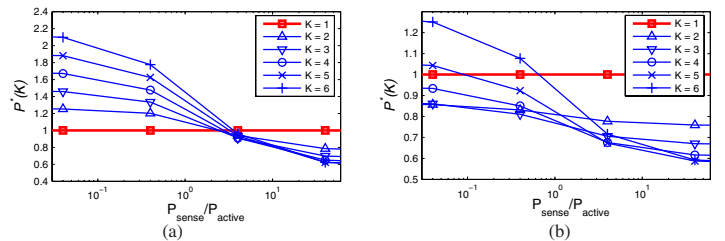
Fig. 9. Normalized optimal network power consumption \mathcal{P}^*(K) vs. \mathcal{P}_{sense}/\mathcal{P}_{active} for (a) message-based and (b) circuit-based inert node model.
