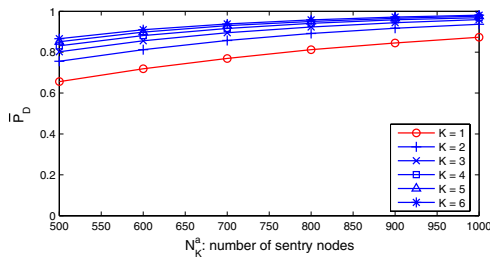
Fig. 4. Expected detection probability ( \bar{P}_D ) vs. number of sentry nodes ( N_K^a ) when P_{FD}^* = 0.001 and N_K^a + N_K^i = 4000 .
