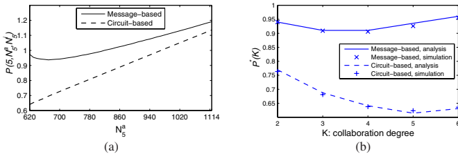
Fig. 8. (a) Given K = 5 , normalized network power consumption ( \mathcal{P}(5, N_s^a, N_s^i) ) vs. number of sentry nodes ( N_s^a ), with N_s^a varying from 620 ( \hat{N}_5^a ) to 1114 ( \hat{N}_1^a ) and the corresponding N_s^i is equal to \hat{N}_5^i(N_s^a) . (b) Normalized optimal network power consumption \mathcal{P}^*(K) for different K and inert node models.
