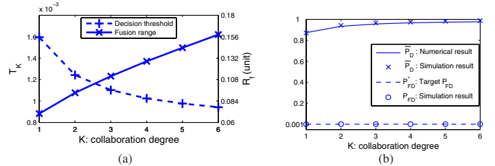
Fig. 6. (a) Normalized decision threshold ( T_K ) and fusion range ( R_f ) when P_{FD} = 0.001 , N_K^a = 1000 , and N_K^i = 3000 . (b) Numerical and simulation results of \bar{P}_D and P_{FD} when P_{FD}^* = 0.001 , N_K^a = 1000 , N_K^i = 3000 , \Omega = 2100 mW, and d_0 = 0.001 units.
