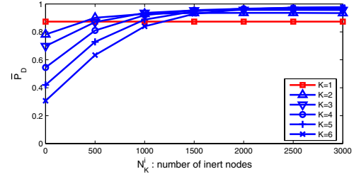
Fig. 5. Expected detection probability ( \bar{P}_D ) vs. number of inert nodes ( N_K^i ) when P_{FD}^* = 0.001 and N_K^a = 1000 .
