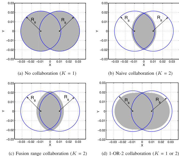
Fig. 3. Coverage region (shown as shaded area) of two active sensors (apart by 0.02 units) in different collaboration scenarios. The detection thresholds used in the four scenarios result in the same P_{FD} . Note that the coverage regions in (b), (c) and (d) are smaller than that in (a).
