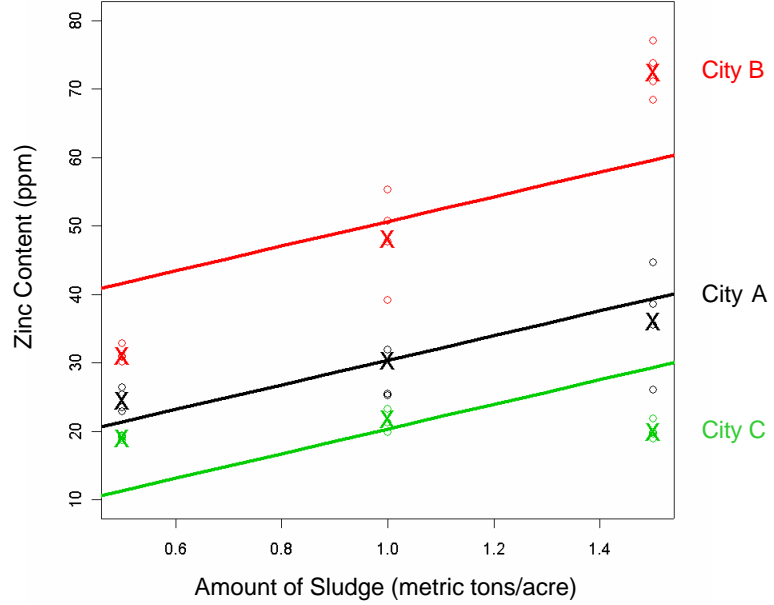
Data with Linear Regression Functions for Each City That Are Constrained to Have the Same Slope (No Interaction)
