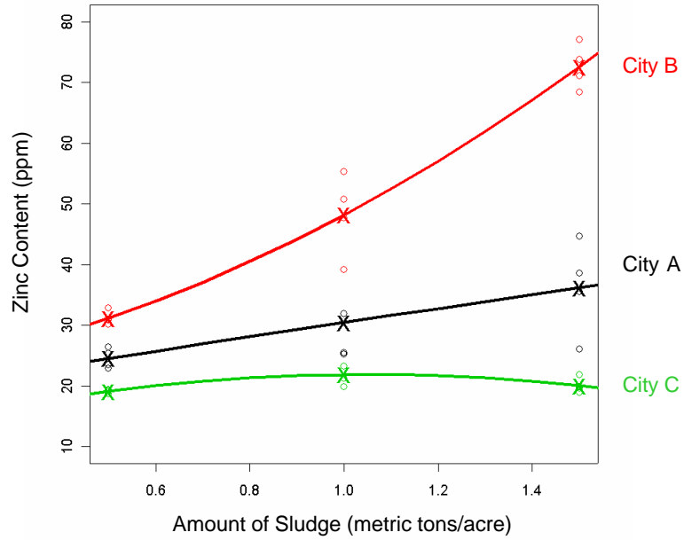
Data with Separate Quadratic Regression Functions for Each City
