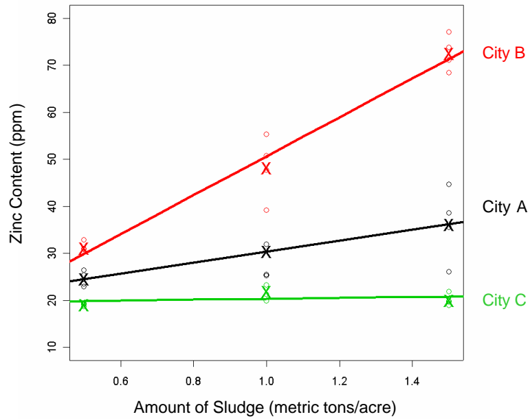
Data with Separate Linear Regression Functions for Each City
