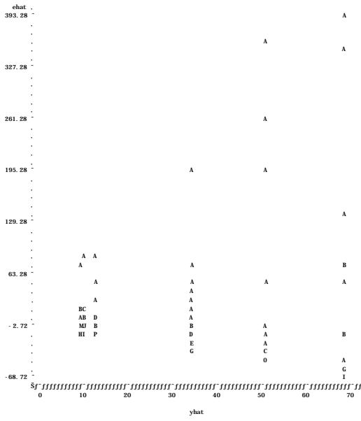
Plot of ehat*yhat. Legend: A = 1 obs, B = 2 obs, etc.
