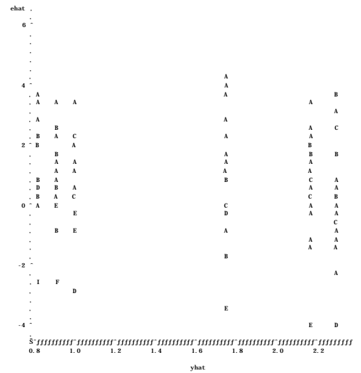
Plot of ehat*yhat. Legend: A = 1 obs, B = 2 obs, etc.
