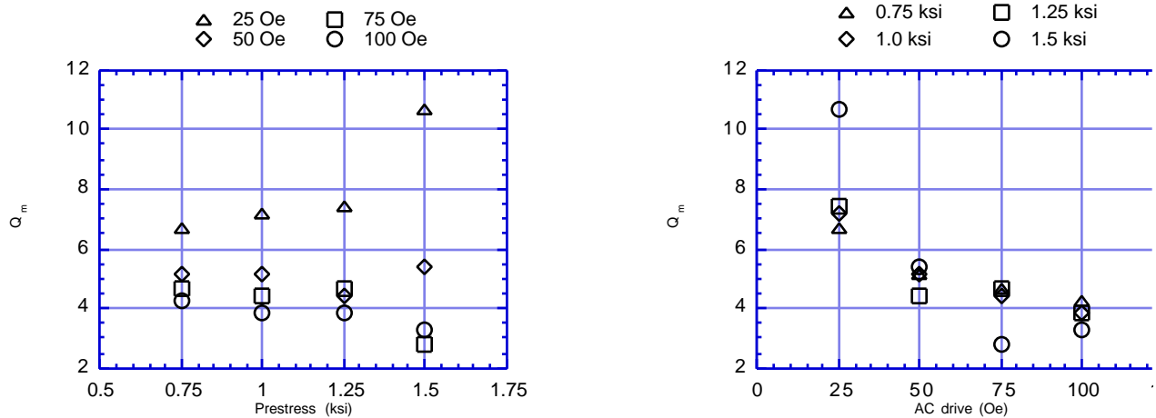
Figure 12a and b: Mechanical quality factor versus a) prestress and b) drive level.
