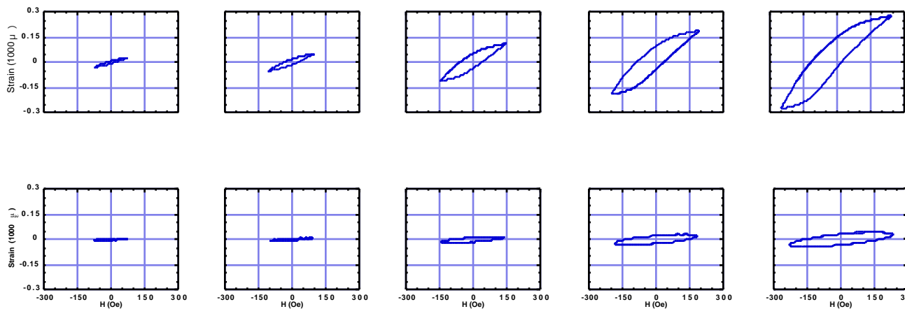
Figure 6: Strain versus H for bias condition 1 (0.75 ksi, 300 Oe) at 0.7 Hz (top set) and 400 Hz (bottom set), AC drive level amplitude increasing from left to right: 75, 100, 150, 200, 250 Oe.
