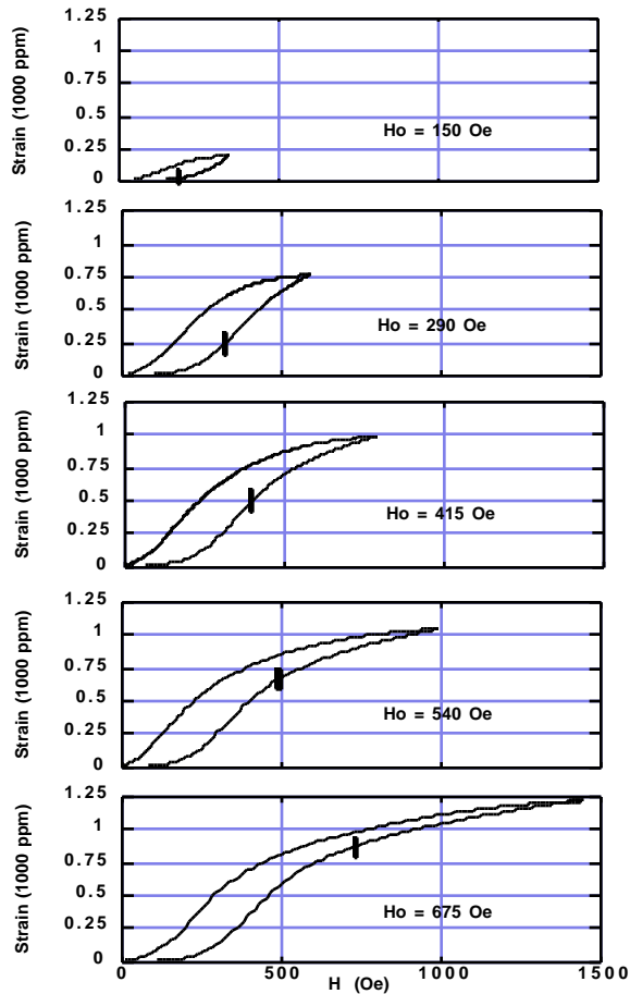
Figure 2: Strain versus applied magnetic field under 1.0 ksi prestress at 150, 290, 415, 540, and 675 Oe. Tick marks indicate magnetic bias H_0 .
