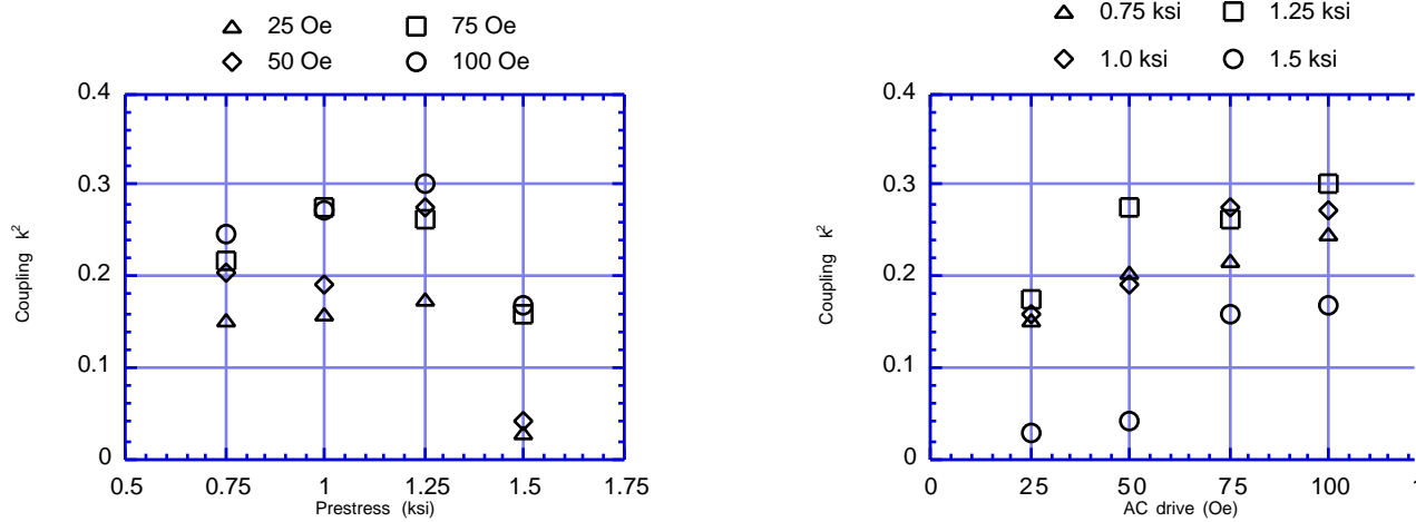
Figures 9a and b: Magnetomechanical coupling versus (a) prestress and (b) drive level.
