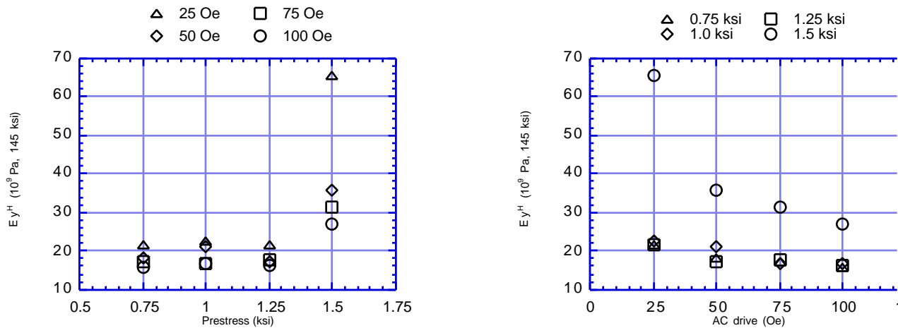
Figures 10a and b: Young's Modulus at constant applied magnetic field versus a) prestress and b) drive level (6.89 MPa = 1.0 ksi).
