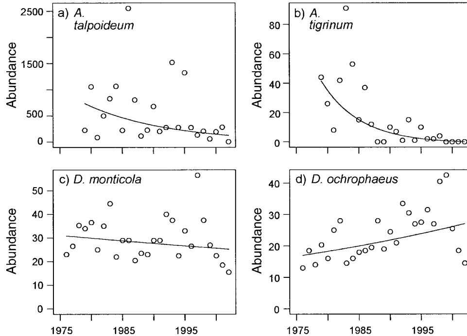
FIG. 1. Trends in number of breeding females for (a) Ambystoma talpoideum and (b) Ambystoma tigrinum over 24 years at Rainbow Bay, Aiken County, South Carolina USA, and in number of amphibians seen in constant-effort searches for (c) Desmognathus monticola and (d) Desmognathus ochrophaeus over 27 years at Coweeta Hydrological Laboratory, Macon County, North Carolina, USA. Lines indicate predicted values from log-linear regressions.
